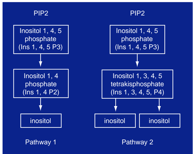
Figure 6. Two major productive pathways for inositol.
