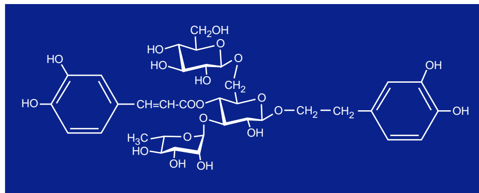
Figure 1. Chemical Structure of Echinacoside
