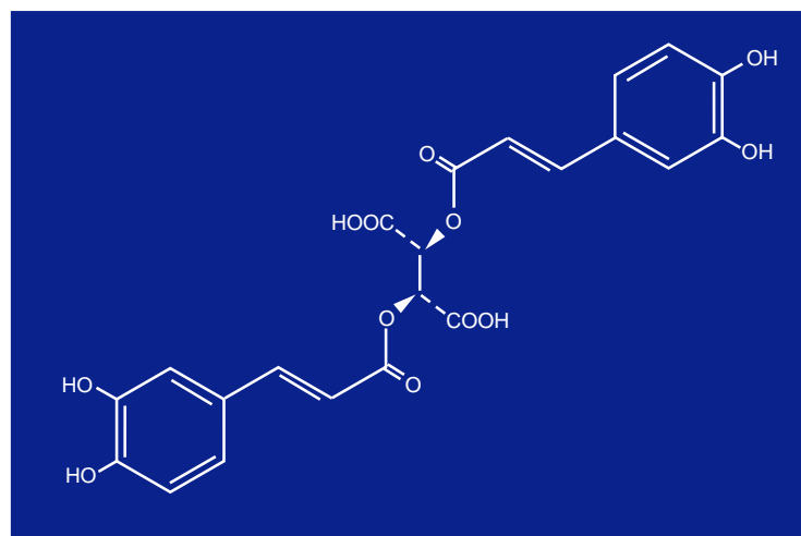
Figure 2. Chemical Structure of Cichoric Acid
